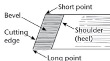
Figure 2. Parts of a skew chisel.
